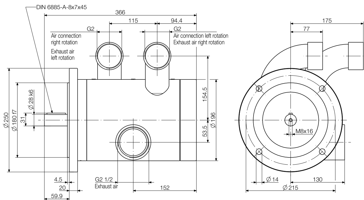
Bracket for motor size 55 and 65 (optional equipment)
