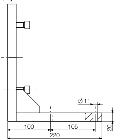
Bracket for motor size 55 and 65 (optional equipment)
