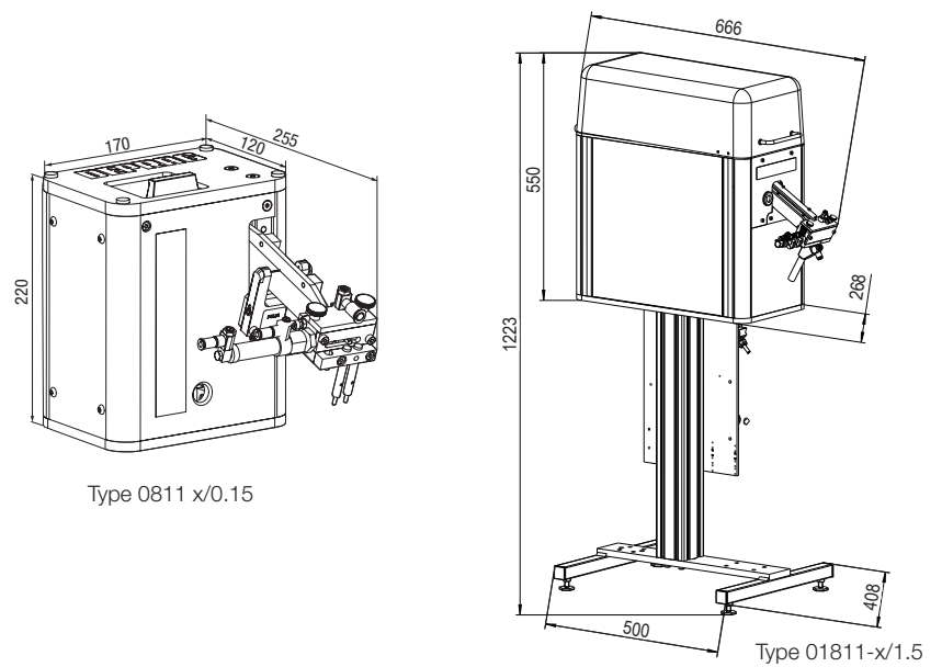
Vibratory Bowl Feeder
